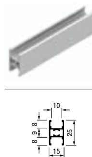
PERFIL CENTRAL RC-BASE "H" HORIZONTAL
